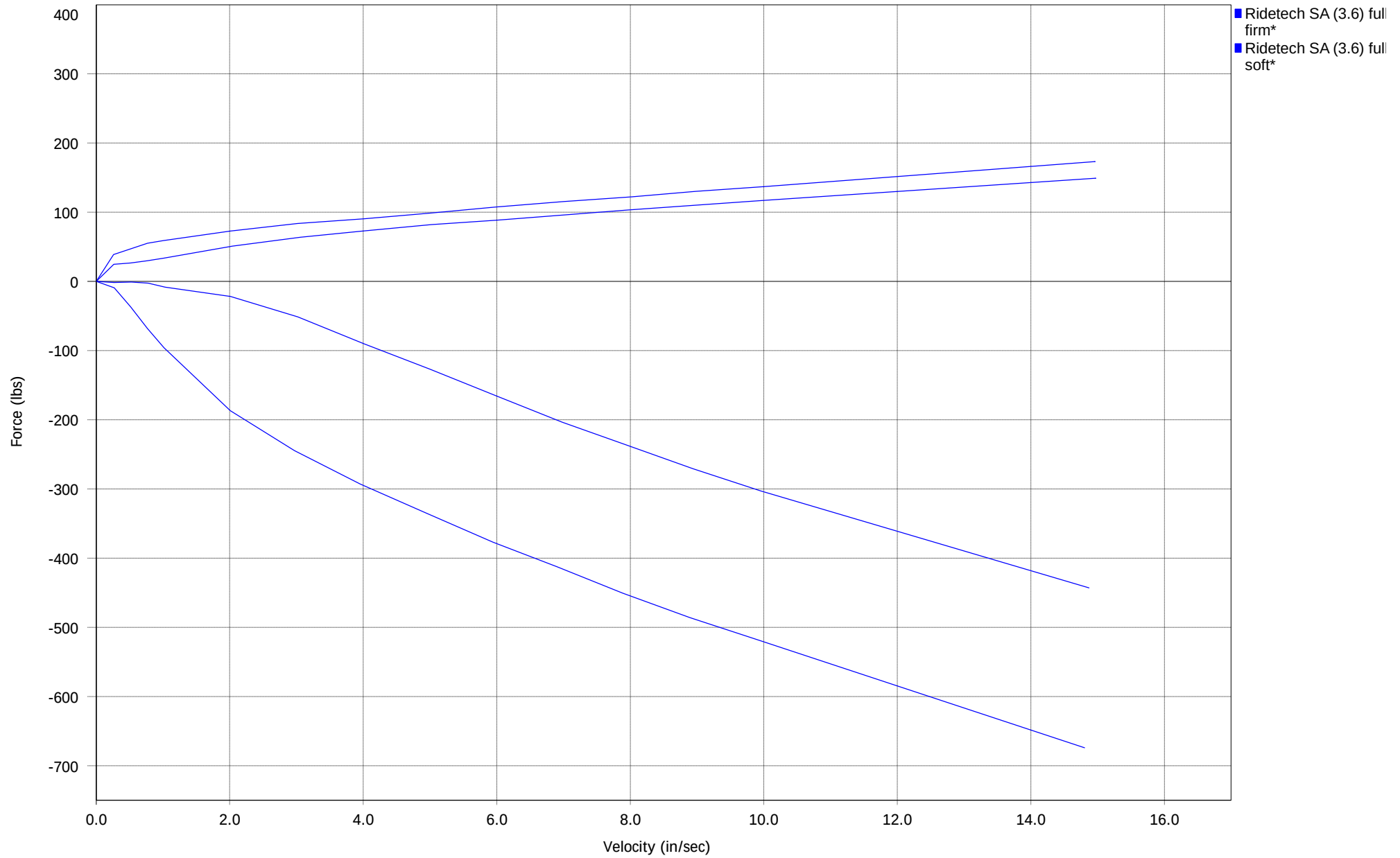
Force Vs. Absolute Velocity
