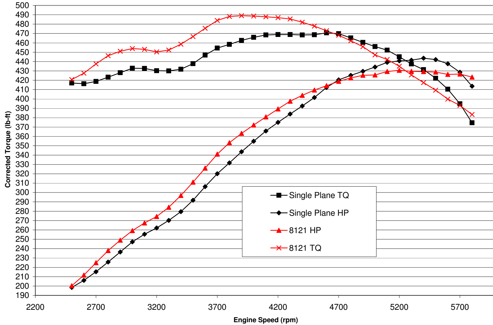
Weiand 8121 vs. GM Single Plane, Stock GM ZZ383
